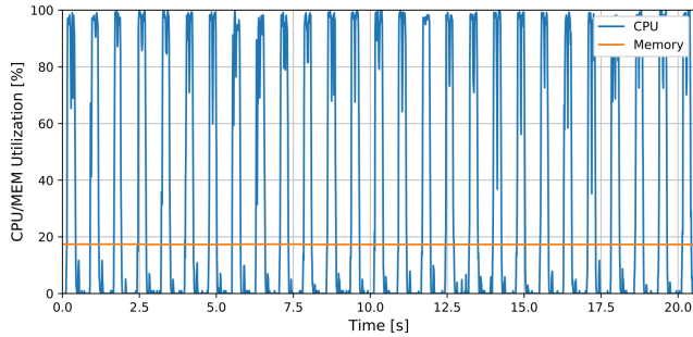
Figure 2: RetinaNet [48] CPU/MEM usage when training on COCO [49] using a GCP TPU v2-8 VM [24].
